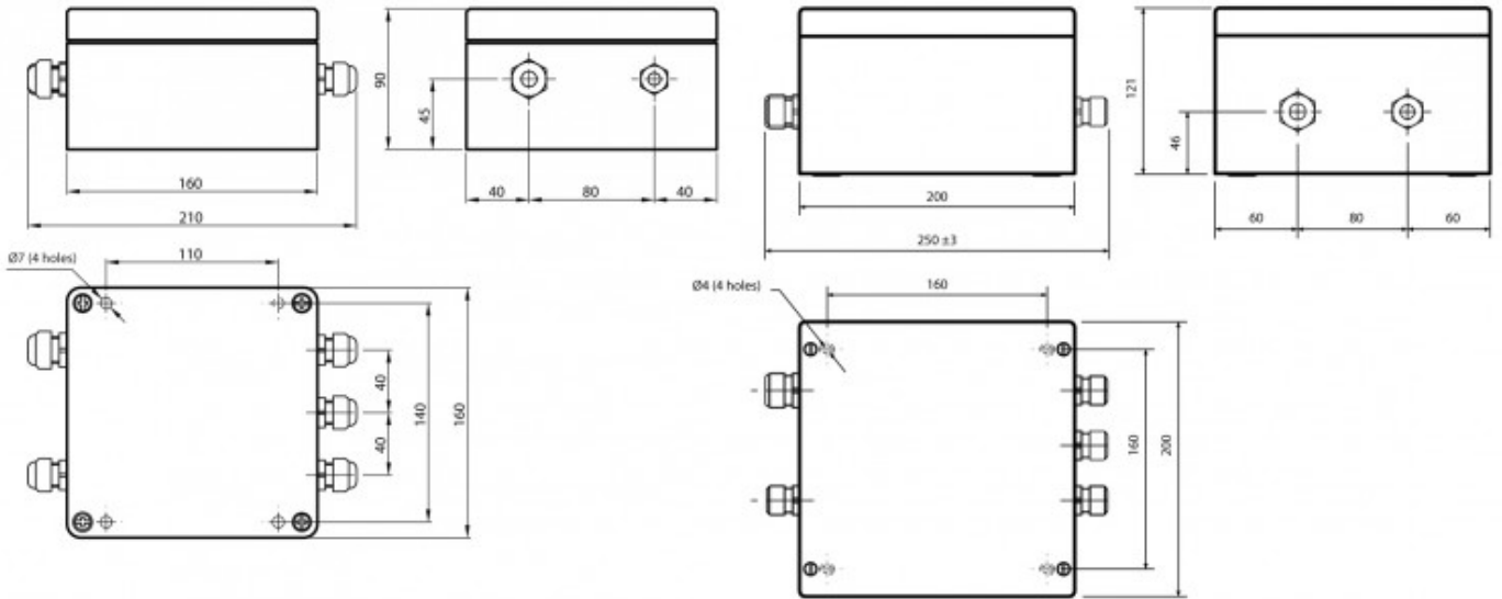
Aluminium housing
